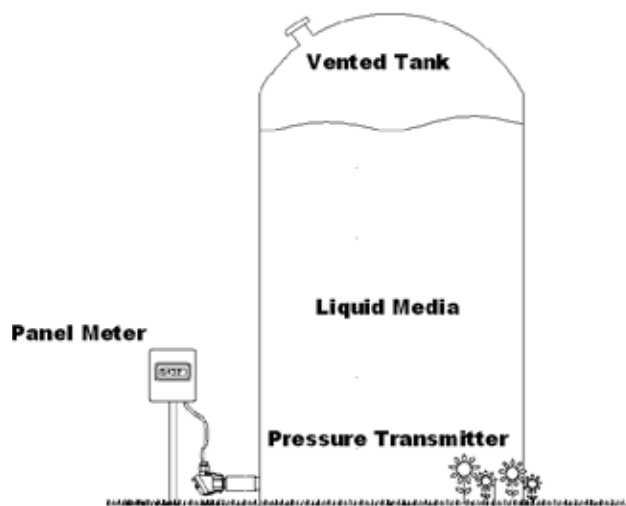
Figure 1: Shows a pipe mount style pressure transmitter. This style transmitter is typically plumbed to the base or side of a vessel & the signal sent to a panel meter or other reading device. This can be utilized where a pipe tap or other mechanical process connection can easily be accessed. A shut-off valve should be utilized for ease of removal.
