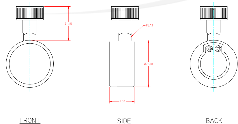
BRWT300 2" WATER TEST GAUGE IN DRAWING SAMPLE
