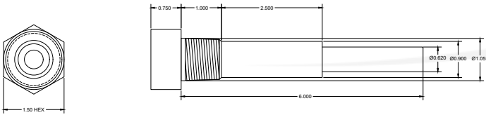
6" Stem without Lag
