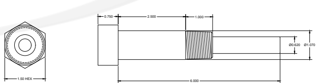
6" Stem with Lag
