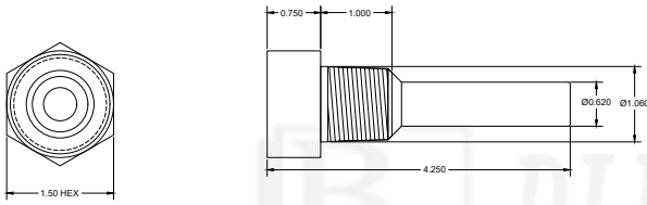
3.5" Stem without Lag
