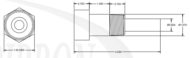
3.5" Stem with Lag
